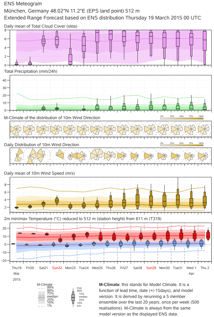
Fig. 10. Example of an ECMWF 15-day ensemble meteogram, depicting time series of surface parameters of a forecast initialized on 19 March 2015 for Munich, Germany. The ensemble distribution is displayed by means of boxplots. This diagram relates forecast daily averages to the model climate (colored background bars). Note how in the daily mean of 10 m wind speed the possibility of high wind speeds on 31 March 2015 (12-day forecast) is predicted (box plot whisker extending over 10 \text{ ms}^{-1} ; the same event as in Fig. 8). (Courtesy of ECMWF.)
